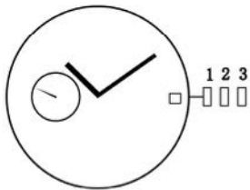
TY2555 (2555) 30 Jewels
